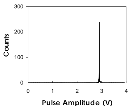
Figure 9: Single photon generated pulse height amplitude spectrum of Geiger mode operated APDs, biased at 3 volts above the breakdown voltage. The avalanche is passively quenched with 100 k \Omega limiting resistors. Assuming the avalanche is triggered by single carriers, the multiplied charge corresponds to a charge gain of 5 \times 10^8 . The narrow peak (FWHM = 0.3%) demonstrates uniform avalanche multiplication across the APD sensitive area.
