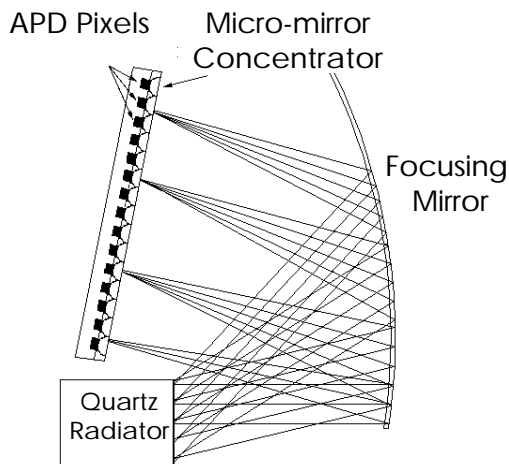
Figure 1: Two-dimensional ray tracing of the optical interface between the quartz radiator and \Delta APD array. A quartz radiator with 1.8 cm vertical dimension, matching the size of DIRC radiators at the BaBar detector [SLAC] was used in the ray tracing geometry. The
