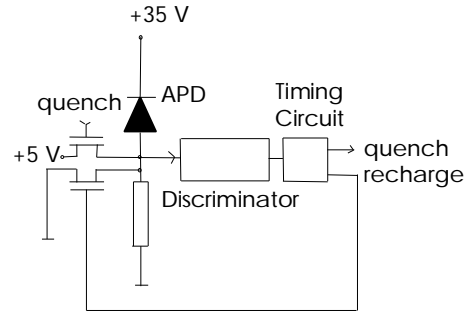
Figure 5: Active circuit configuration.
