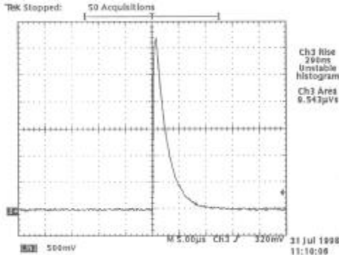
Figure 3: Geiger pulse shape for passive quenching with a limiting (quenching) resistor (horizontal scale 5 \mu sec/div, vertical scale 500mV/div, bias 45.5 volts). The peak current pulse is 33 \mu A and the corresponding gain is 5 \times 10^8 .
