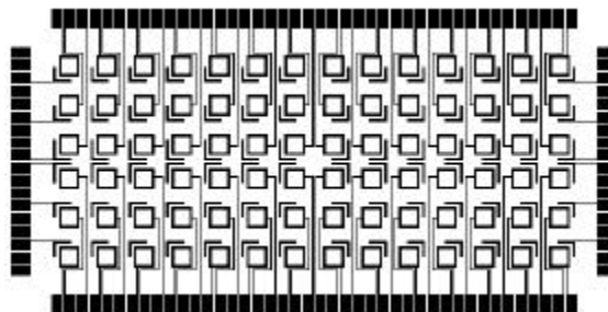
Figure 2: Layout of the interconnection layer for 6 x 14 pixels \Delta APD array. All pixels in a row will have the anodes connected to the lateral pads (row isolation). The cathodes of each APD are wired to the pads lined on the long sides of the rectangle. The pitch size is 300 \mu m and the APD active area is 150 \mu m x 150 \mu m.
