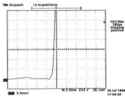
Figure 4: Leading edge of the Geiger pulse for 100 K limiting resistor (horizontal scale 2.5 nsec/div, vertical scale 5 mV/div). The slew rate is approximately 30 V/ \mu sec. Low threshold detection (30 mV) may result in less than 2 nsec time delay.
