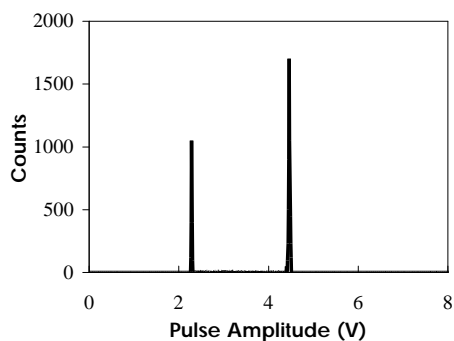
Figure 10: Pulse height amplitude spectrum of Geiger mode operated APDs, operated with pulsed bias above the breakdown voltage. The first peak (left) is due to the charging current only (no Geiger events), while the second peak is due to Geiger and charging currents through APD.
