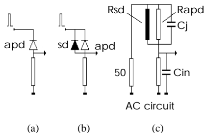
Figure 7(a): Schematic of the pulsed bias with resistive load; (b) Schottky diode (sd) connected in parallel with the \mu APD sinks more charge to ground during the charge recovery period (pulsed bias OFF); (c) Equivalent ac circuit, showing the parasitic elements of the
